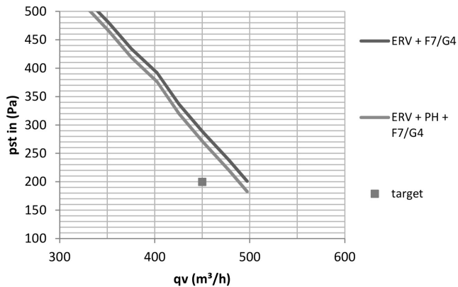
Air performance
